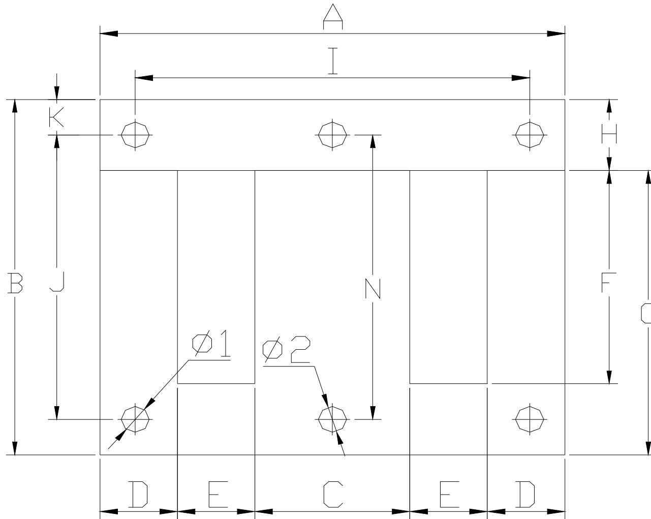
EI lamination Drawing
